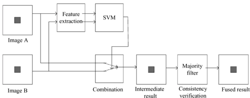
Fig. 2. Schematic diagram of the proposed fusion method.
