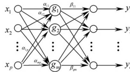
Fig. 1. The topological structure of PPLN
