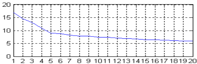
Fig. 6. The graph of logarithm of the largest 20 eigenvalues
