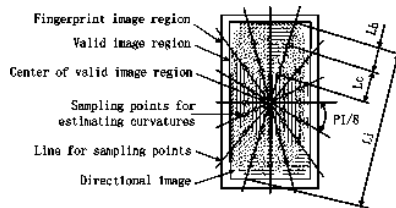
Fig. 1. Location of sampled points in directional image
