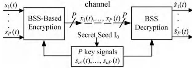
Fig. 1. Block diagram of BSS-based encryption method
