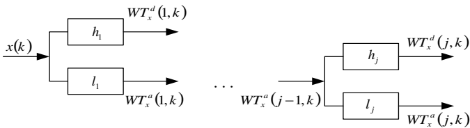
Fig. 1. Calculation algorithm of SWT.
