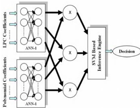
Fig. 3.6. FFT-LPC-PAC parallel MLP diagram
