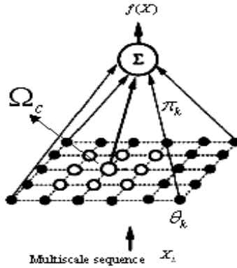
Fig. 2. The structure of the multiscale self-organizing mixture network
