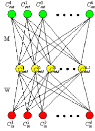
Fig. 3. Two-layer neural network classification
