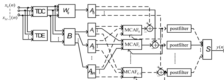
Fig. 1. Structure of microphone array based speech enhancement algorithm
