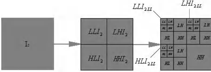
Fig. 1. Wavelet analysis of facial illumination compensation
