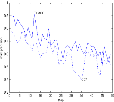
Fig. 4. The precision of CC4 and TextCC (2 corner)
