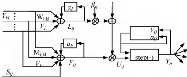
Fig. 2. PCNN neuron model
