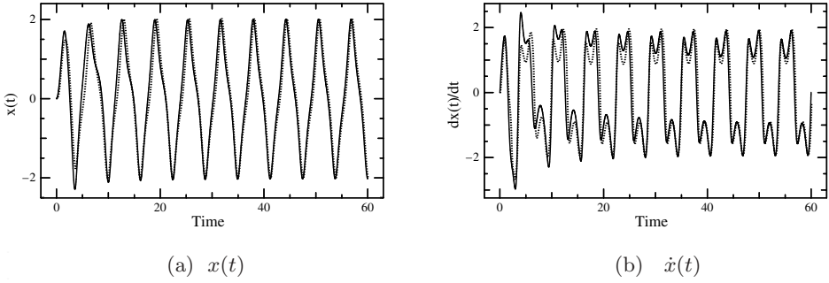
Fig. 2. Comparison of output of Duffing's equation and its DRNN model (— : output of Duffing's eq.; ··· : output of DRNN)
