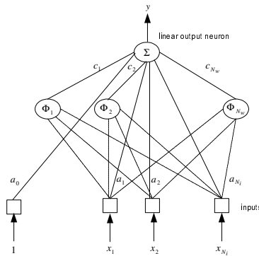
Fig. 2. Wavelet network structure
