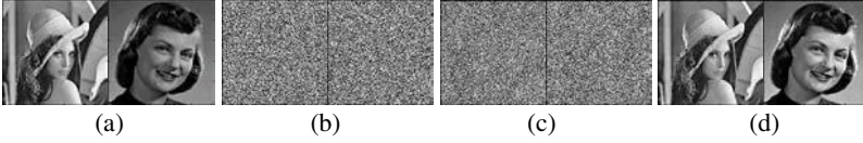
Fig. 2. Example of BSS-based encryption of two original images ( P=2 , T=65536 ). (a) Two original images s_1(t) and s_2(t) . (b) Two key images s_{n1}(t) and s_{n2}(t) . (c) Two encrypted images x_1(t) and x_2(t) . (d) Two decrypted images \hat{s}_1(t) and \hat{s}_2(t) with Comon’s algorithm
