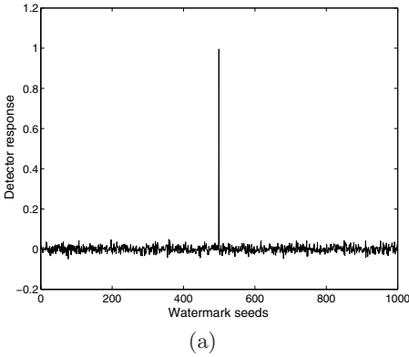
Fig. 3. Detector response for 1000 watermark seeds
