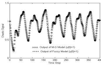
Fig. 2. Training result of model ( \tau=17 )
