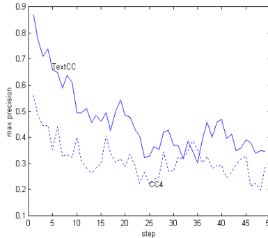
Fig. 5. The precision of CC4 and TextCC (4 corner)
