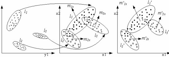
Fig. 1. From left to right, Left shows the y in L is divided into 3 clusters. Middle is the corresponding x clusters according to y . Right is the x' clusters in subspace.
