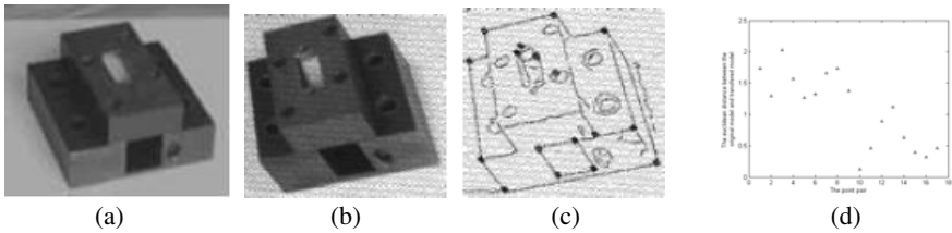
Fig. 3. Matching results of the transformed model against the model image (Affine parameters are computed by the point pairs) (a) The original image of the model with \theta = 0^\circ , t = 0^T ; (b) The transferred model of the left image with the parameters: A = \begin{bmatrix} 0.8082 & 0.6203 \\ -0.3765 & 0.8352 \end{bmatrix} , t = \begin{bmatrix} -0.3765 \\ 86.6797 \end{bmatrix} ; (c) The edge model with corners; (d) The matching error of the affine model images.
