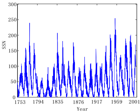
Fig. 2. Time series of raw sunspots data
