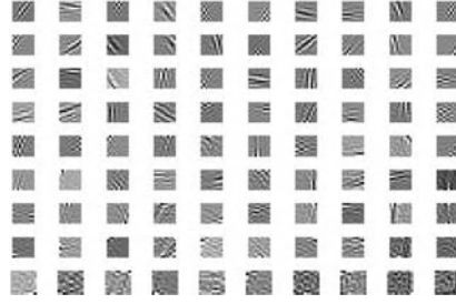
Fig. 1. 90 ICA filters obtained by training an ensemble of 10 \times 10 natural image patches
