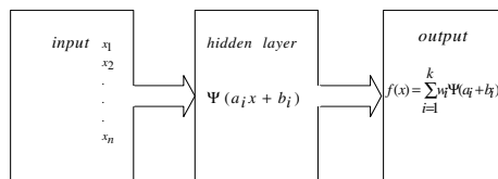
Fig. 1. The structure of a wavelet network as the one of the neuron
