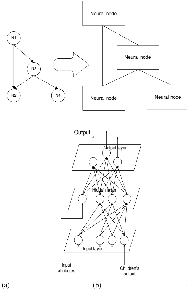
Fig. 2. An illustration of a data structure with its nodes encoded by a single-hidden-layer neural network. (a) A Directed Acyclic Graph (DAG); (b) The encoded DAG; (c) The illustration of the neural network.
