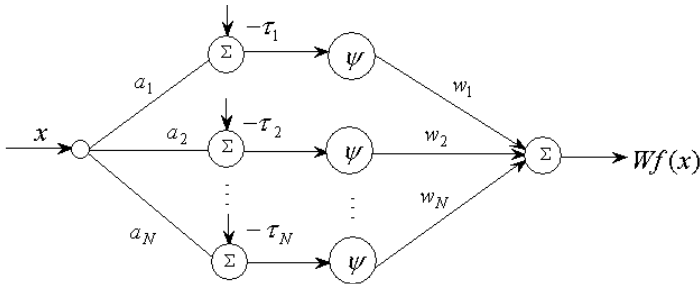
Fig. 2. Structure of wavelet neural network
