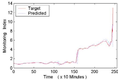
Fig. 2. Filed gear tooth prognostic result
