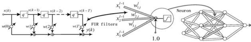
Fig. 1. Structure of FIRNN
