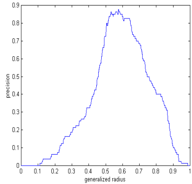
Fig. 3. The influence of radius on precision of TextCC
