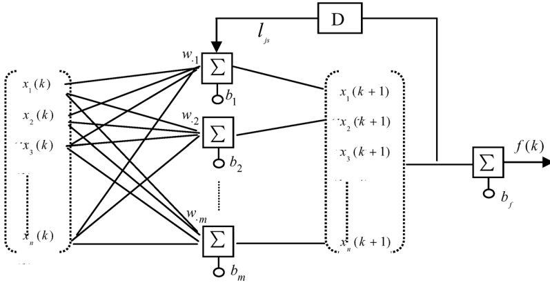
Fig. 2. Architecture of Elman neural network
