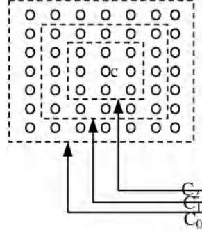
Fig. 2. Topological neighborhood
