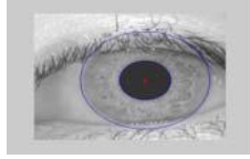
Fig. 2. Localized image
