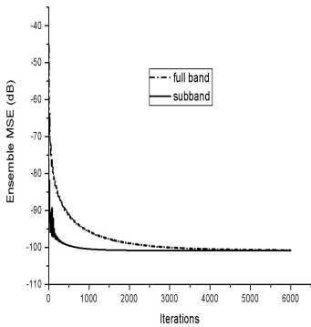
Fig. 2. Learning curves
