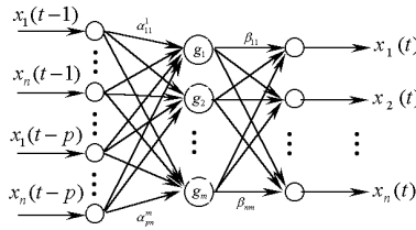
Fig. 2. The topological structure of the PPLN for n -dimensional NLAR ( p )
