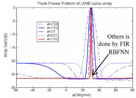
Fig. 5. The peak power directivity pattern of using FIR and RBF NN
