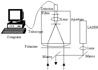
Fig. 2.1. Diagram of Lidar configuration
