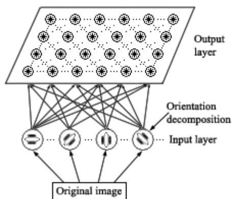
Fig. 1. The structure of the neural network
