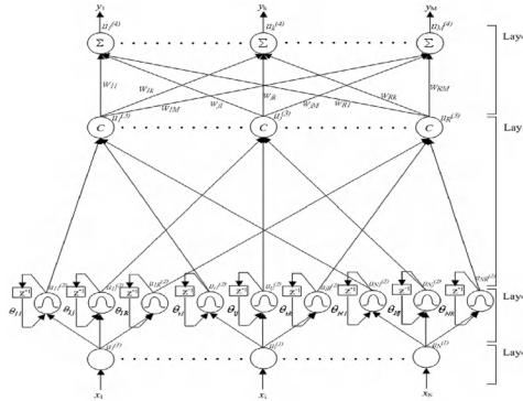
Fig. 1. Structure of the proposed RCNFS
