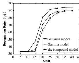
Fig. 2. The average recognition rates versus the SNR
