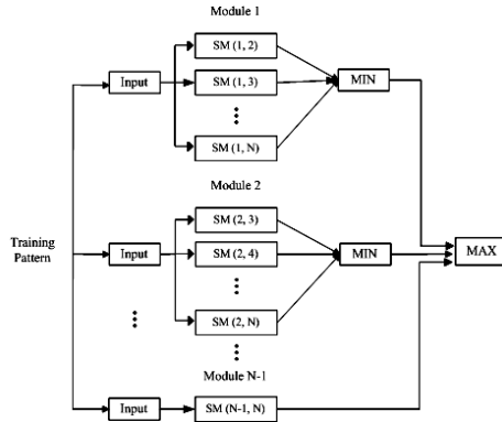
Fig. 1. The architecture of the modular neural network, where “SM” denotes “Sub-Module”
