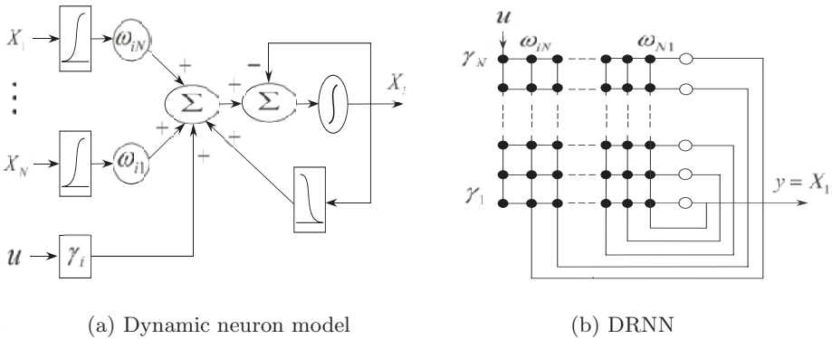
Fig. 1. Architecture of dynamic neural network
