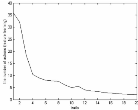
Fig. 4. Times to reach optimal feature set versus number of test
