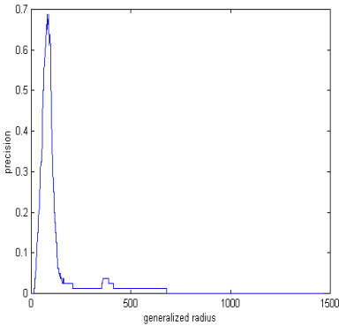
Fig. 2. The influence of radius on precision of CC4
