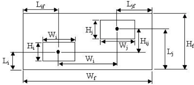
Fig. 2. Geometrical relation of Eye-pair Candidates
