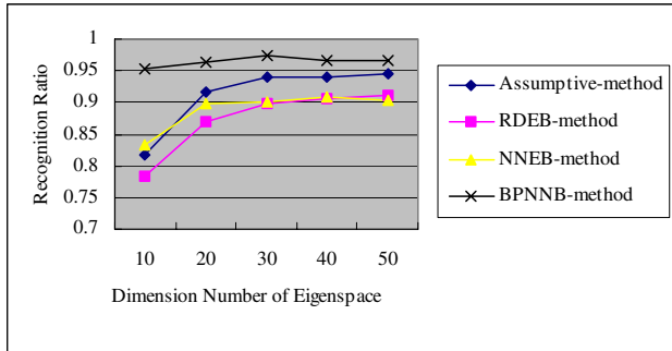
Fig. 4. Recognition Performance
