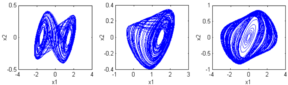
Fig. 1. Different chaotic attractors of 3-order CNN model. (a) a_1 = 3.86 , s_{11} = -1.55 , s_{12} = 8.98 , s_{32} = -14.25 ; (b) a_1 = 3.85 , s_{11} = -1.55 , s_{12} = 8.76 , s_{32} = -14.35 ; (c) a_1 = -4.198 , s_{11} = 2.365 , s_{12} = 7.45 , s_{32} = -10.98
