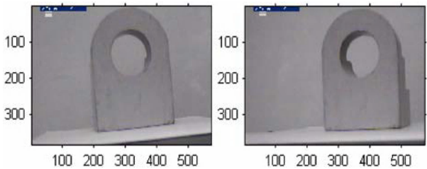
Fig. 4. Original image
