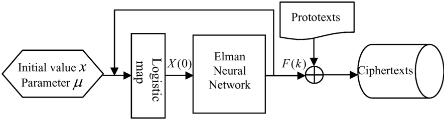
Fig. 3. Cooperation between chaotic encryption and Elman neural network
