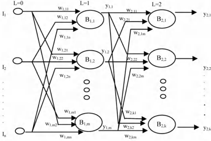
Fig. 3. A multi-layer feedforward net structure
