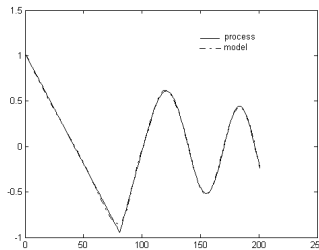
Fig. 5. Nonlinear static model and process outputs
