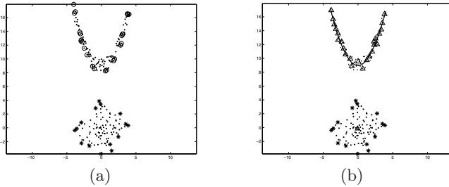
Fig. 2. The clustering result of the mixed data set with a spherical cluster and a parabola-shaped cluster
