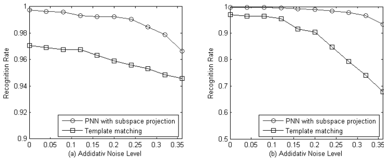
Fig. 5. Recognition rate versus additive noise level. (a) Only testing images corrupted by noise. (b) Both training and testing images corrupted by noise
