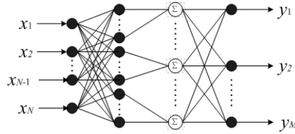
Fig. 1. The topology scheme of radial basis probabilistic neural network
