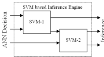
Fig. 4.1. SVM based IE
