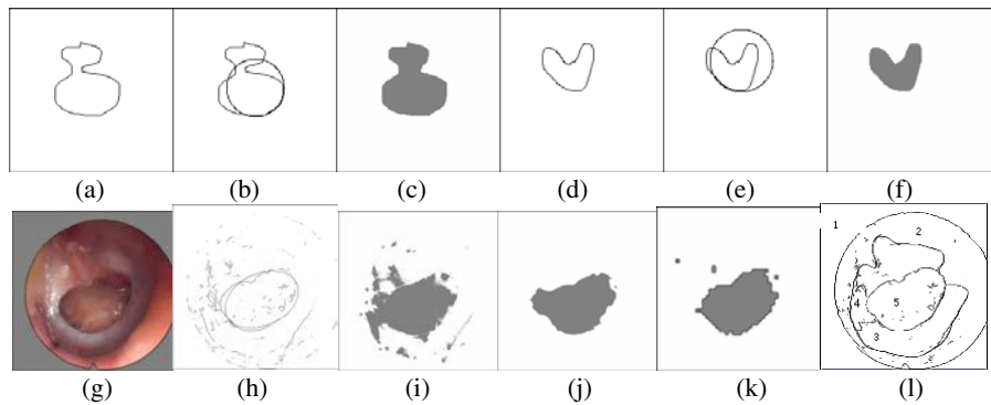
Fig. 4. The random calabash shape and the created results: (a) the original calabash image. (b) the result of Hough Transform. (c) the result of Radar Algorithm. (d) the original heart image. (e) the result of Hough Transform. (f) the result of Radar Algorithm. (g) the original eardrum image. (h) the result of Hough Transform. (i) the result of Narrow-sensed Radar Algorithm. (j) the result of Multi-Step Narrow-sensed Radar Algorithm. (k) the result of Vision Model method. (l) the result using Broad-sensed Radar Algorithm to extract regions
