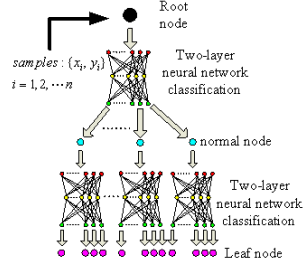
Fig. 4. Modified HDR tree structure
