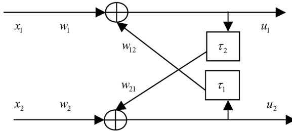
Fig. 2. Separation network for delayed mixtures
