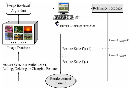
Fig. 2. Feature learning of HCI-based reinforcement learning and relevance feedback
