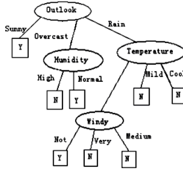
Fig. 1. The final decision tree model of ID3 algorithm
